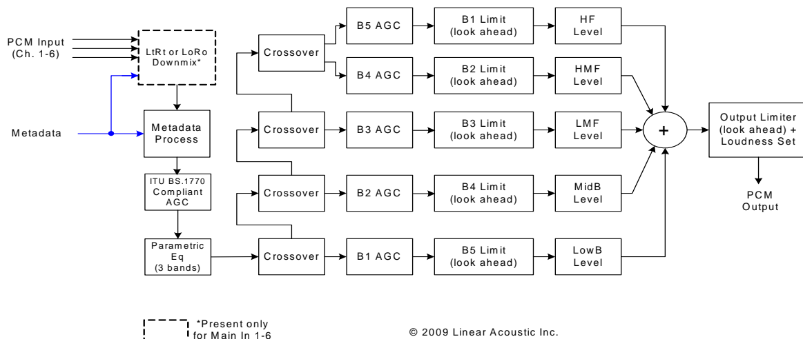
Figure 7-1 General signal flow of the AERO.one processing core
