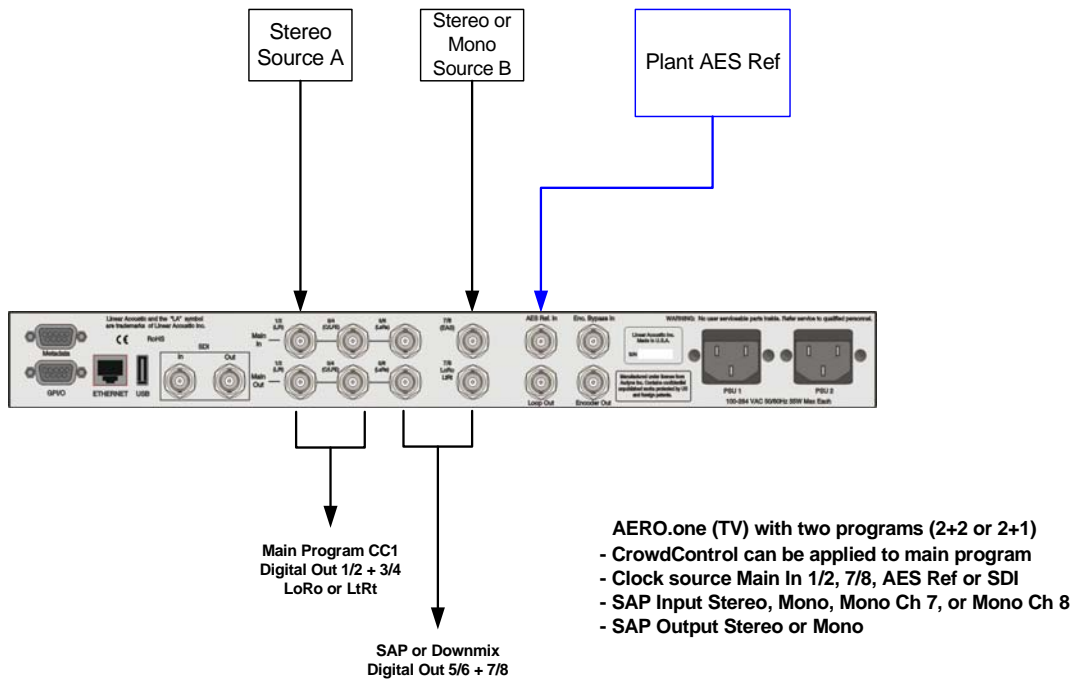
Figure 3-2 AERO.one(TV) accepting 2 + 2 or 2 + 1 audio.
