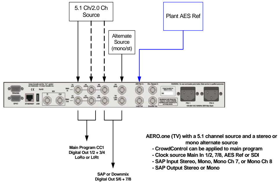
Figure 3-3 AERO.one(TV) accepting 5.1 + 2 audio.
