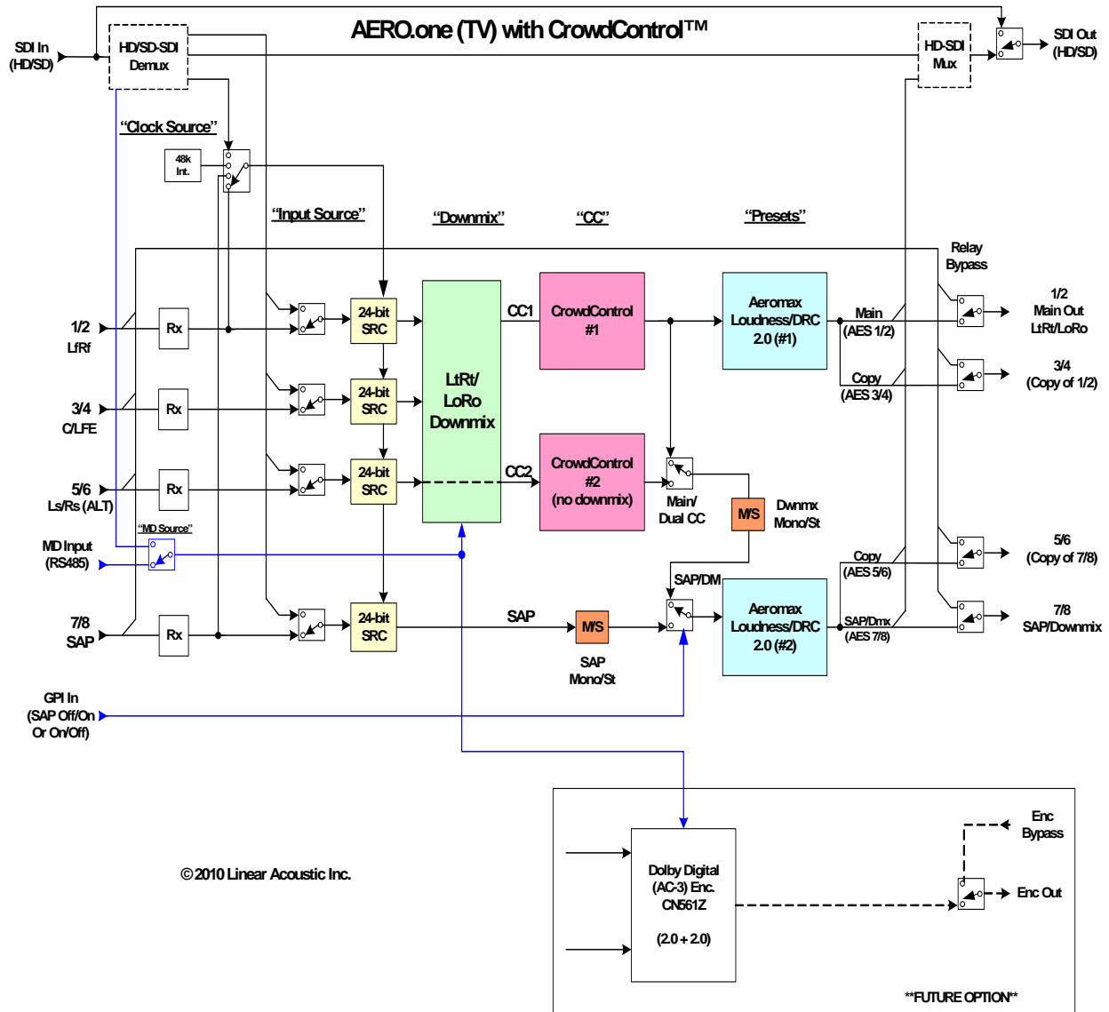
Figure 1-1 Basic Audio Block Diagram with SDI and Crowd Control
